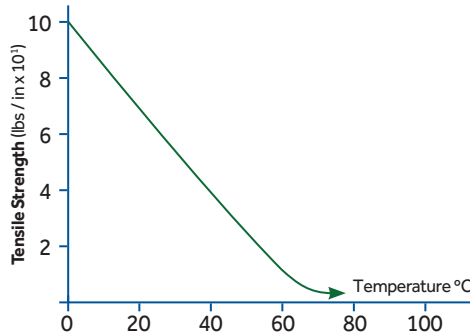
Relationship between Tensile Strength & Temperature
