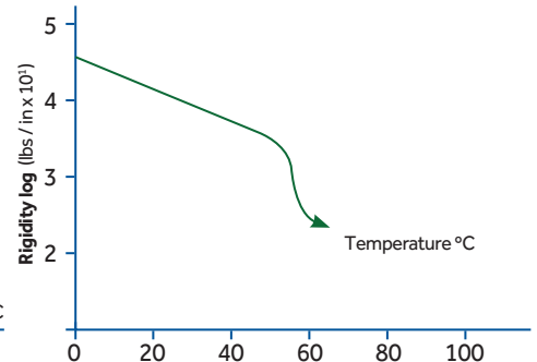
Relationship between Rigidity & Temperature
