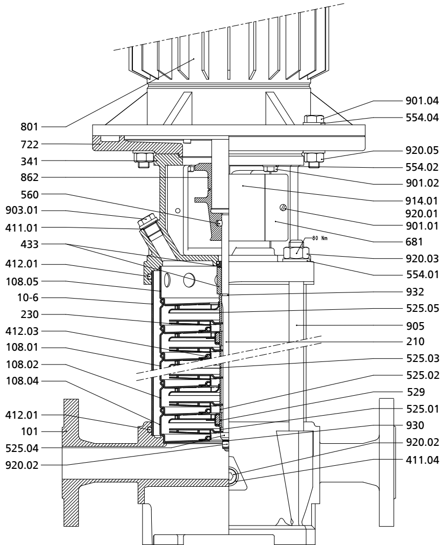
General assembly drawing of Movitec LHS 6
