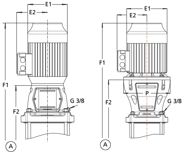
Movitec VF/VSF; VCF Motor version V18
