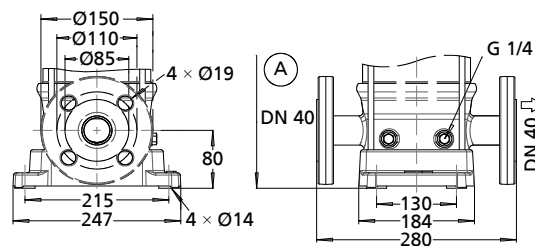
Movitec VCF
