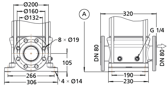
Movitec VF/VSF - interchangeable range
